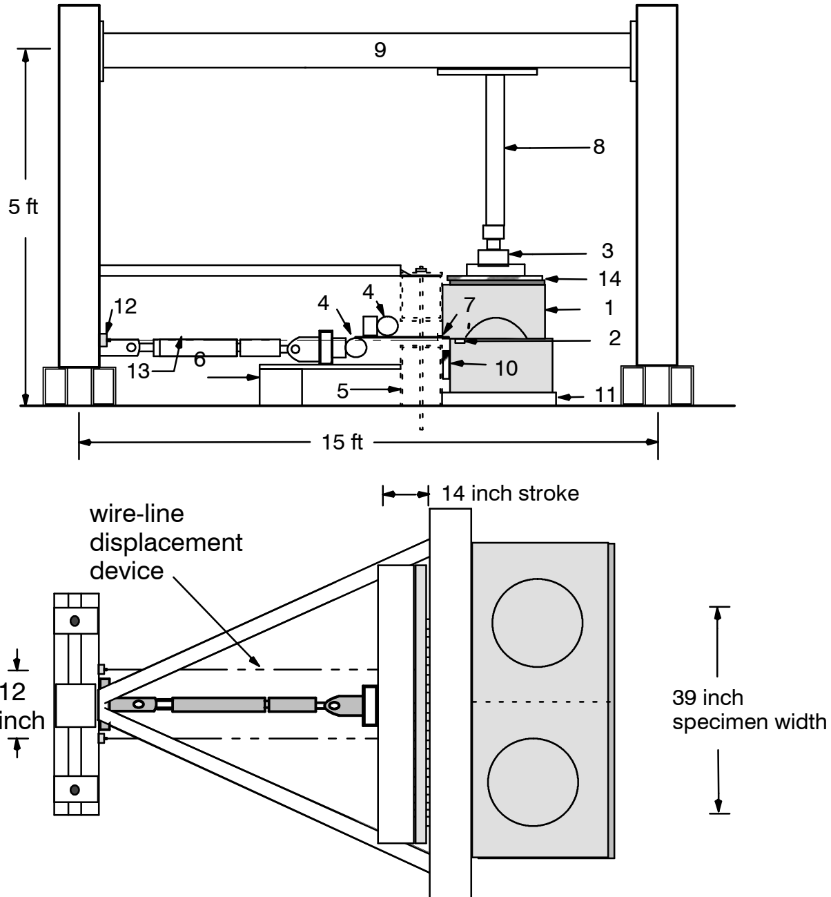
Figure 1: Schematic of connection test apparatus showing Redi-Rock units and Miragrid 8XT geogrid using the anchored tail configuration
