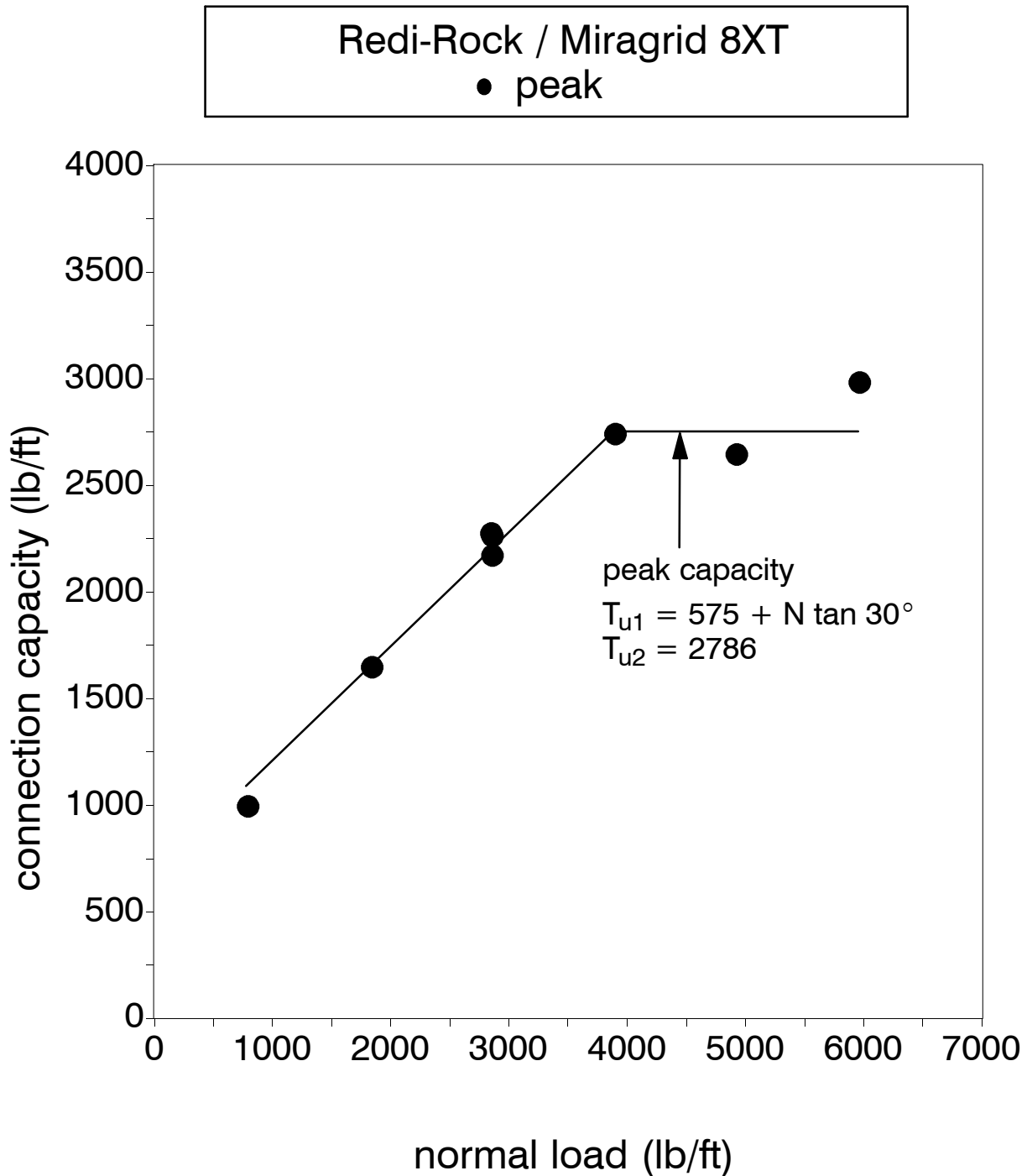
Figure 3: Connection capacity versus normal load for Redi-Rock block with one 7/16 inch diameter fiberglass connector rod and Miragrid 8XT using the anchored tail configuration
