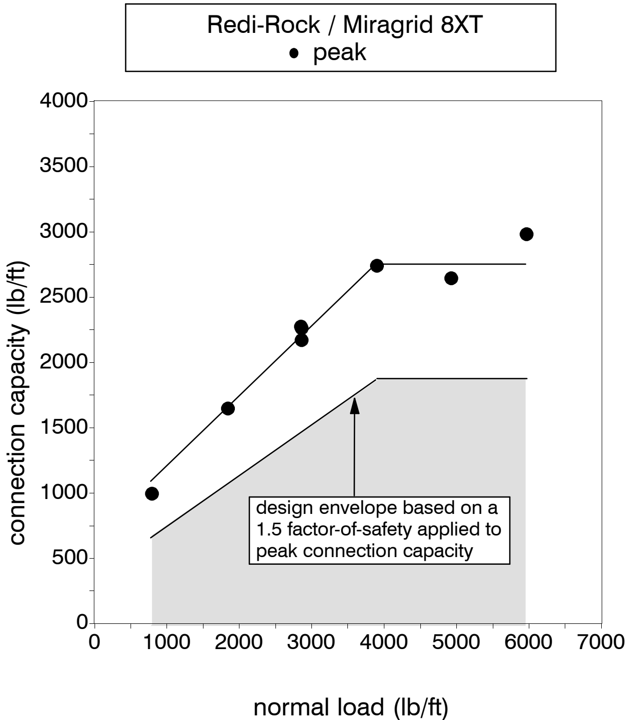
Figure 4: Preliminary design capacity envelope for Redi-Rock modular block units with one 7/16 inch diameter connector rod and Miragrid 8XT geogrid combination using the anchored tail configuration
